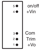
Pinning S9-1 Dual Output
