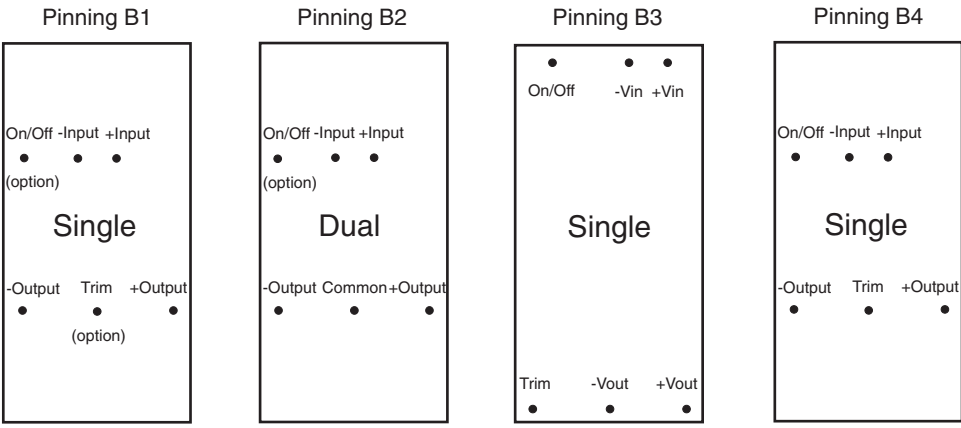
"B" cases, bottom view
