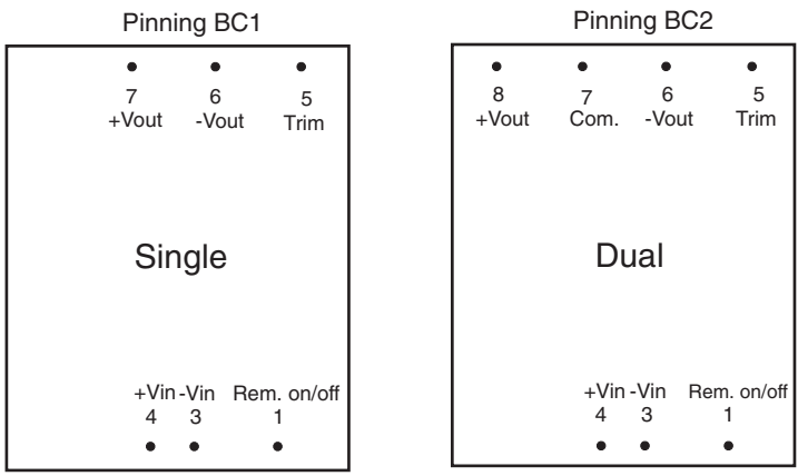
"BC" cases, bottom view
