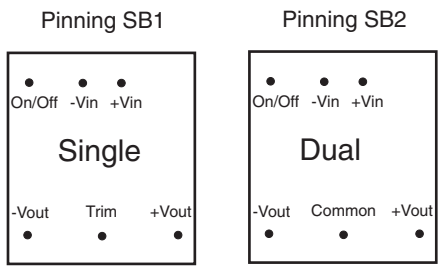
"SB" cases, bottom view
