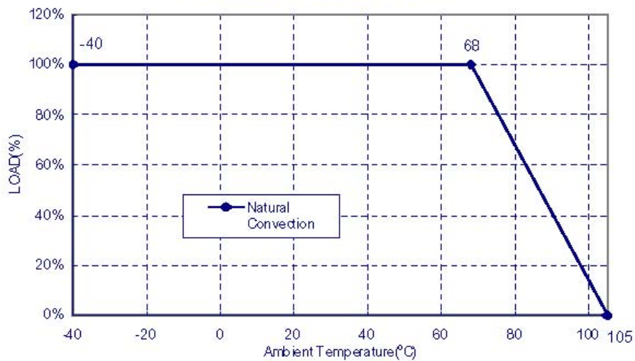
Typical Derating curve for Natural Convection
